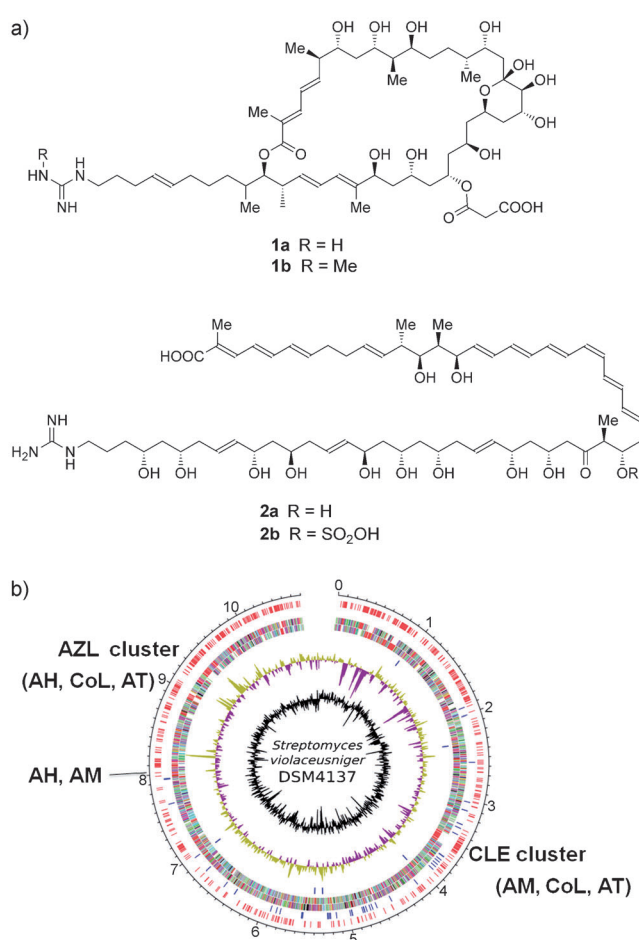
Figure 1. a) The structures of the guanidine-containing antibiotics azalomycin [F3a ( 1a ) and F4a ( 1b )] and desulfoclethramycin ( 2a ) and clethramycin ( 2b ) produced by Streptomyces violaceusniger DSM 4137; b) the location of the corresponding azl and cle gene clusters, and of candidate genes for the synthesis and attachment of their common 4-guanidinobutanoyl starter unit, on the S. violaceusniger chromosome. AM, flavin-dependent arginine 2-monooxygenase (decarboxylating); AH, 4-guanidinobutyramide hydrolase; CoL, 4-guanidinobutanoate:CoA ligase; AT, 4-guanidinobutyryl-CoA:ACP acyltransferase.
